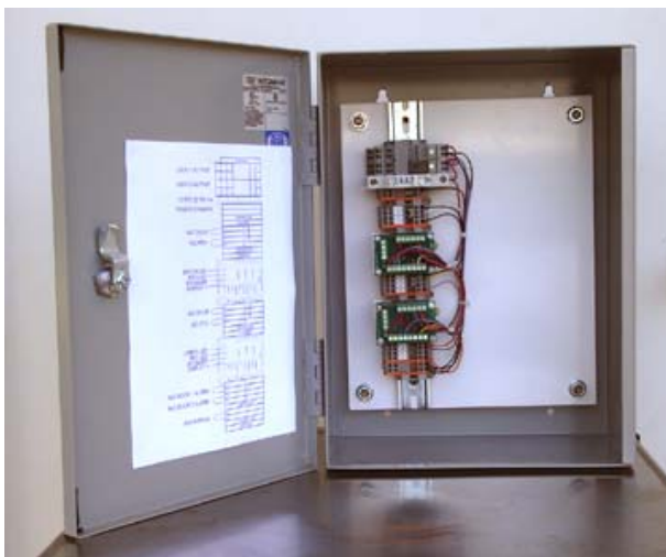
System Electronics Mounted in Enclosure
